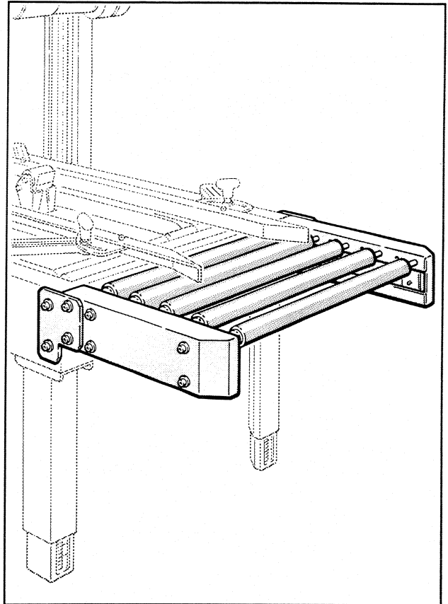
P/N 78-8055-0951-6 – Conveyor Extension Attachment – Shown installed on 77A-KS Adjustable Case Sealer
