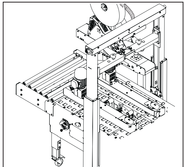
Exit Conveyor Extension Attachment
