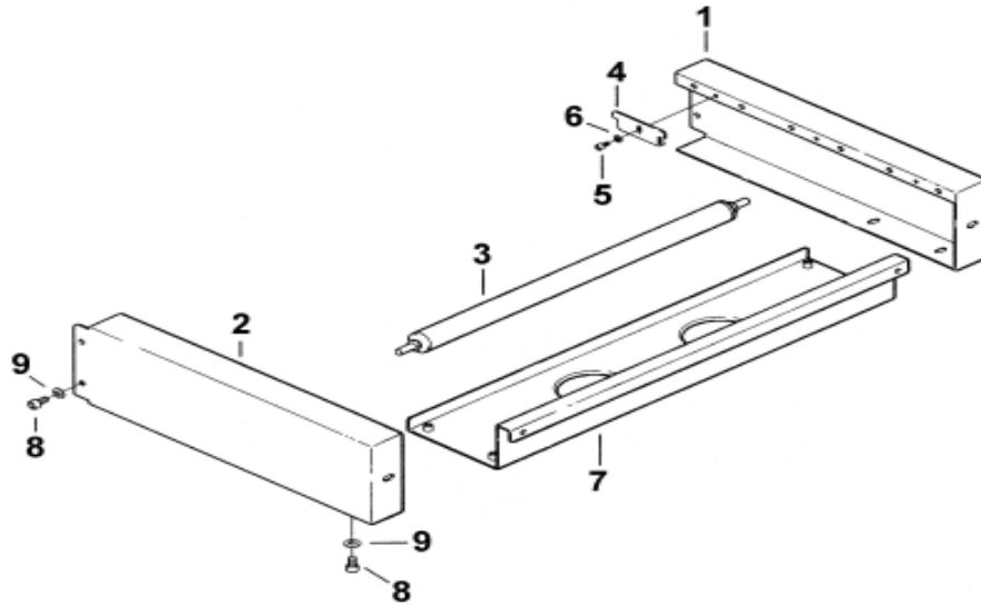
Figure 2 – Parts Illustration
